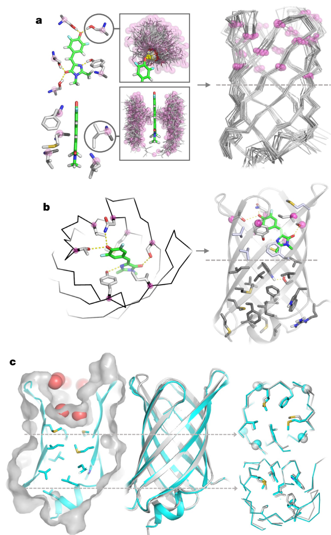
Fig. 3 | Computational design and structural validation of \beta -barrels with recessed cavities for ligand binding. a , Left, ensembles of side chains generated by the RIF docking method making hydrogen-bonding (upper left) and hydrophobic interactions (lower left) with DFHBI (green); pre-generated interacting rotamers are shown in grey with backbone C_{\alpha} highlighted by magenta spheres. Right, ensemble of 200 \beta -barrel backbones with C_{\alpha} atoms surrounding the binding cleft indicated by magenta spheres. b , Each ligand-scaffold pair (left) with multiple ligand-coordinating interactions from RIF docking is subjected to Rosetta energy-based sequence design calculations (right): positions around the ligand (light purple, above the dashed line) are optimized for ligand binding; the bottom of the barrel (dark grey, below the dashed line), for protein stability. c , Left, crystal structure (cyan cartoon with grey surface) of b10 with a recessed binding pocket filled with water molecules (red spheres). Middle, b10 design model backbone (silver) superimposed on the crystal structure (cyan). Right, comparison of crystal structure and design model for two different barrel cross-sections (indicated by dashed lines); glycine C_{\alpha} atoms are indicated by spheres in the upper layer.
