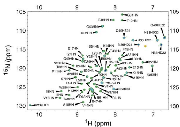
Figure 5. ^1H - ^{15}N HSQC spectrum of CFr. The HSQC spectrum of \sim 1 mM ^{15}N -CFr in 50 mM phosphate buffer (pH 7.0), recorded at 298 K and 500 MHz. 81 Peaks are labelled with the one-letter amino acid code and sequence number.
