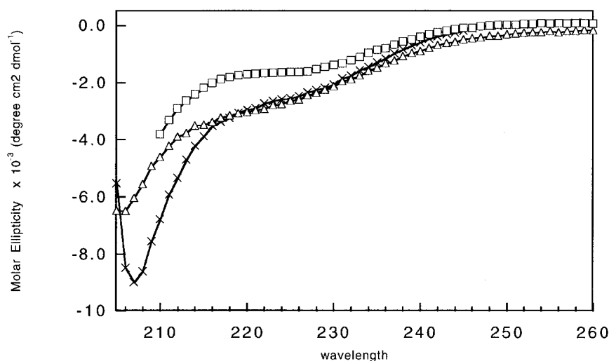
Figure 3. CD spectra of 283, 290, and 425 sequences in isolation. Spectra of 283 (△), 290 (□), and 425 (crosses) were taken in 100 mM sodium phosphate (pH 7), 50 mM NaCl and 120, 20, and 250 mM guanidine, respectively. Protein concentrations were 20 \pm 0.4 \mu M.
