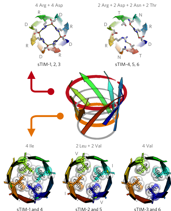
Figure 3 | Effect of two-fold- versus four-fold-symmetrical barrel interior on stability. Starting from the sTIM-1 sequence, we explored variations in the interior of the \beta -barrel. The different packing layers of the barrel are shown with circles in the central barrel figure. Models for two of the layers where asymmetric designs were made are shown in red and orange. Two configurations were tested for the polar red layer and three for the hydrophobic orange layer. The six possible combinations were tested with variants sTIM-1–sTIM-6. For example, sTIM-1 is four-fold symmetrical with four arginine-aspartate salt bridges crowning the top (red layer) and has four isoleucines in the interior of the barrel (orange layer). Strands are sequentially colored from blue to red, and for the orange layer configurations, side chain packing is shown with space-fill spheres. The stabilities of the six different variants correlate strongly with the configurations in the hydrophobic packing layer, in the order sTIM-1 (71.9 °C) \approx sTIM-4 (71.8 °C) > sTIM-2 (66.5 °C) \approx sTIM-5 (65.8 °C) > sTIM-6 (59.3 °C) \approx sTIM-3 (56.9 °C). (CD melting curves of these variants are provided in Supplementary Fig. 5.)
