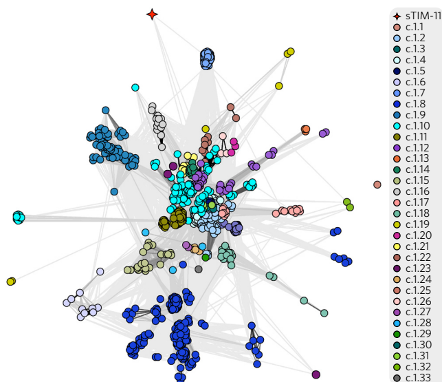
Figure 5 | Sequence relationships between natural ( \beta/\alpha ) 8 -barrels and sTIM-11. HHsearch calculations with sTIM-11 against the Astral SCOPe 2.04 database filtered for 95% sequence identity were carried out, and clustering was performed at a P -value cutoff of 1.0 \times 10^{-2} . Connections are shown in different shades of gray with a linear scaling between P values of 1.0 \times 10^{-2} and 1.0 \times 10^{-56} .
