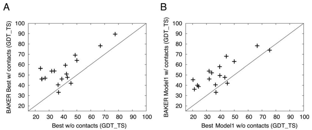
Figure 4. Contact assisted predictions are significantly improved over most nonassisted predictions based on GDT-TS scores. (A) Best BAKER contact assisted predictions versus the best nonassisted predictions among all predictor groups for the 17 target domains (the GDT-TS scores for Tc658-D1 and Tc684-D2 are close enough to appear as the same point). (B) Model 1 BAKER contact assisted predictions versus the best model 1 nonassisted predictions among all predictor groups for the 17 target domains.
